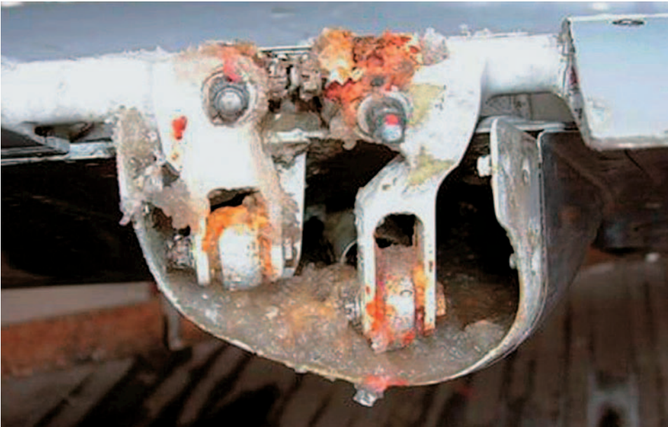
Figure 1: Elevator control
